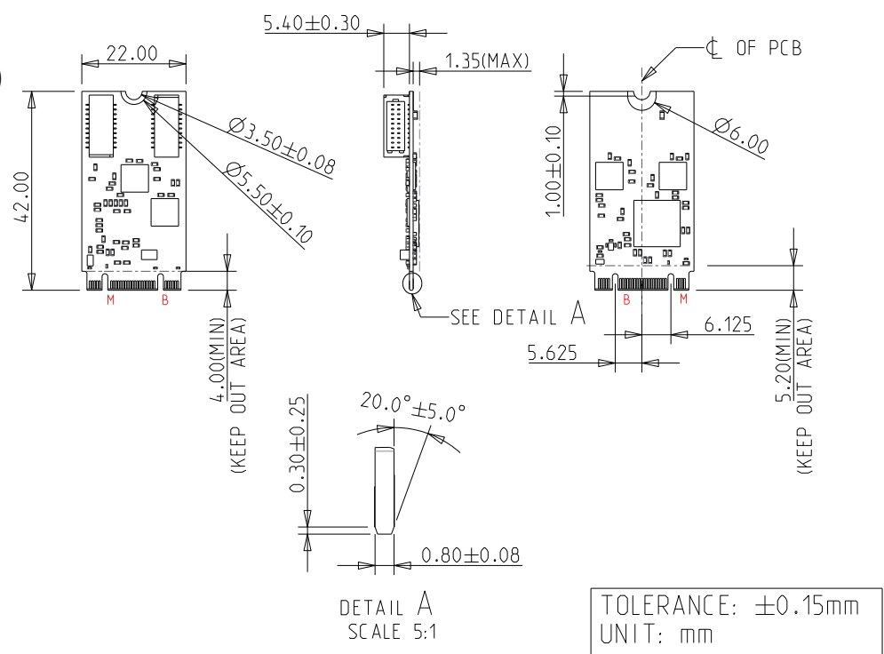
EGP2-X403-W2 (Horizontal Connector)
