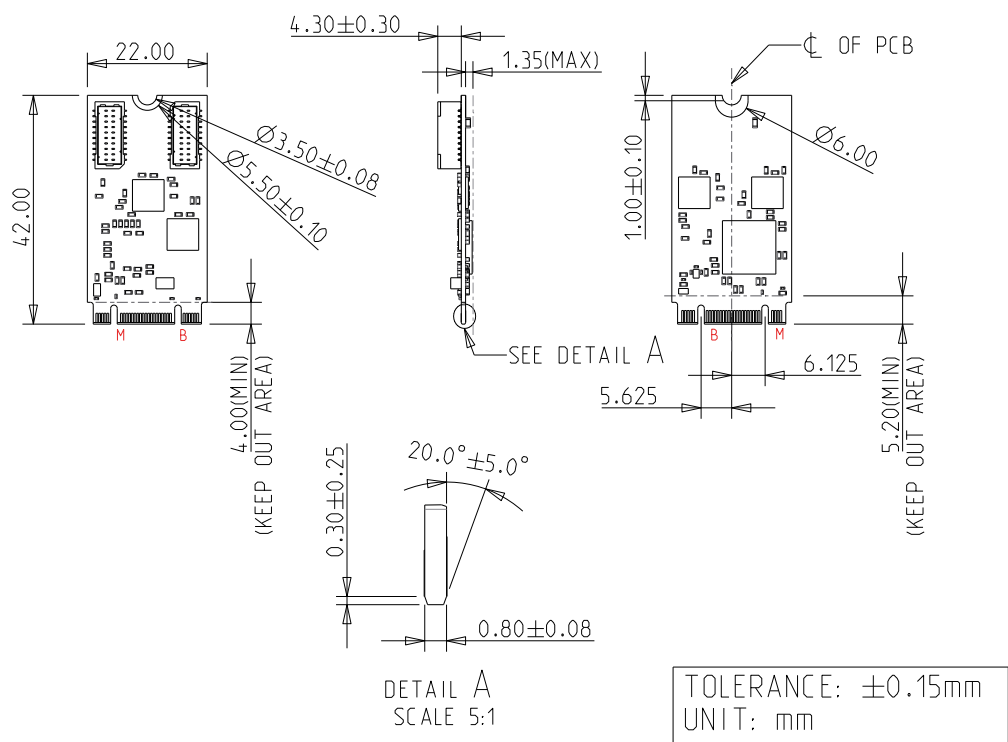
EGP2-X403-W1 (Vertical Connector)
